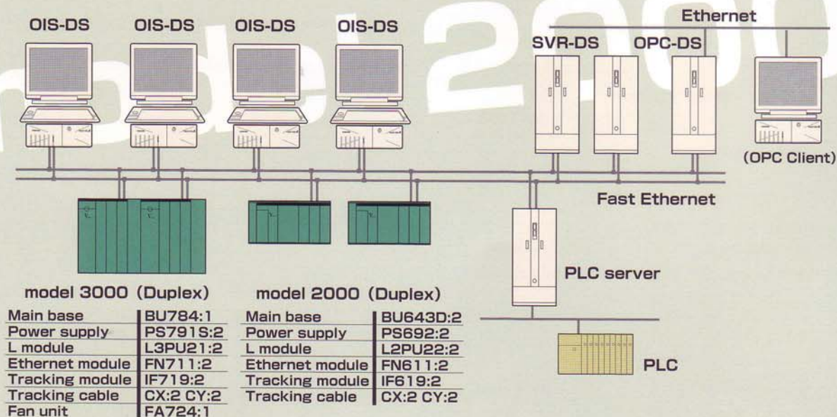
TOSDIC-CIE DS system configuration example
